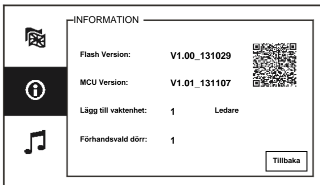
Fig. 23 Systeminformation
